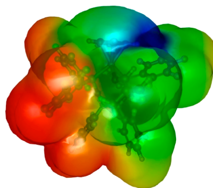
Figure 5. Molecular electrostatic potential of the methacrolein–( R,R )-1 complex A .
