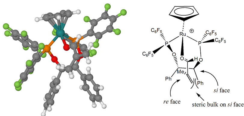
Figure 3. Structure A of the complex-( R,R )-1 with one molecule of methacrolein and the proposed approach of the nitrene.
