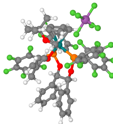
Figure 7. Methacrolein–( R,R )- 1 –MTBE– \text{SbF}_6^- complex.
