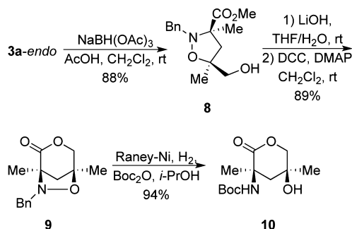
Scheme 4. Synthesis of 3-Amino-5-hydroxy Lactone 10
