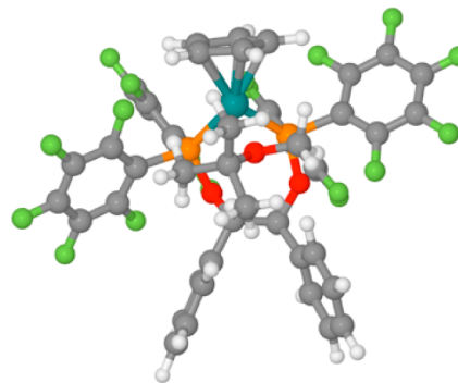
Figure 2. Structure of the complex-( R,R )- 1 with one molecule of MTBE.
